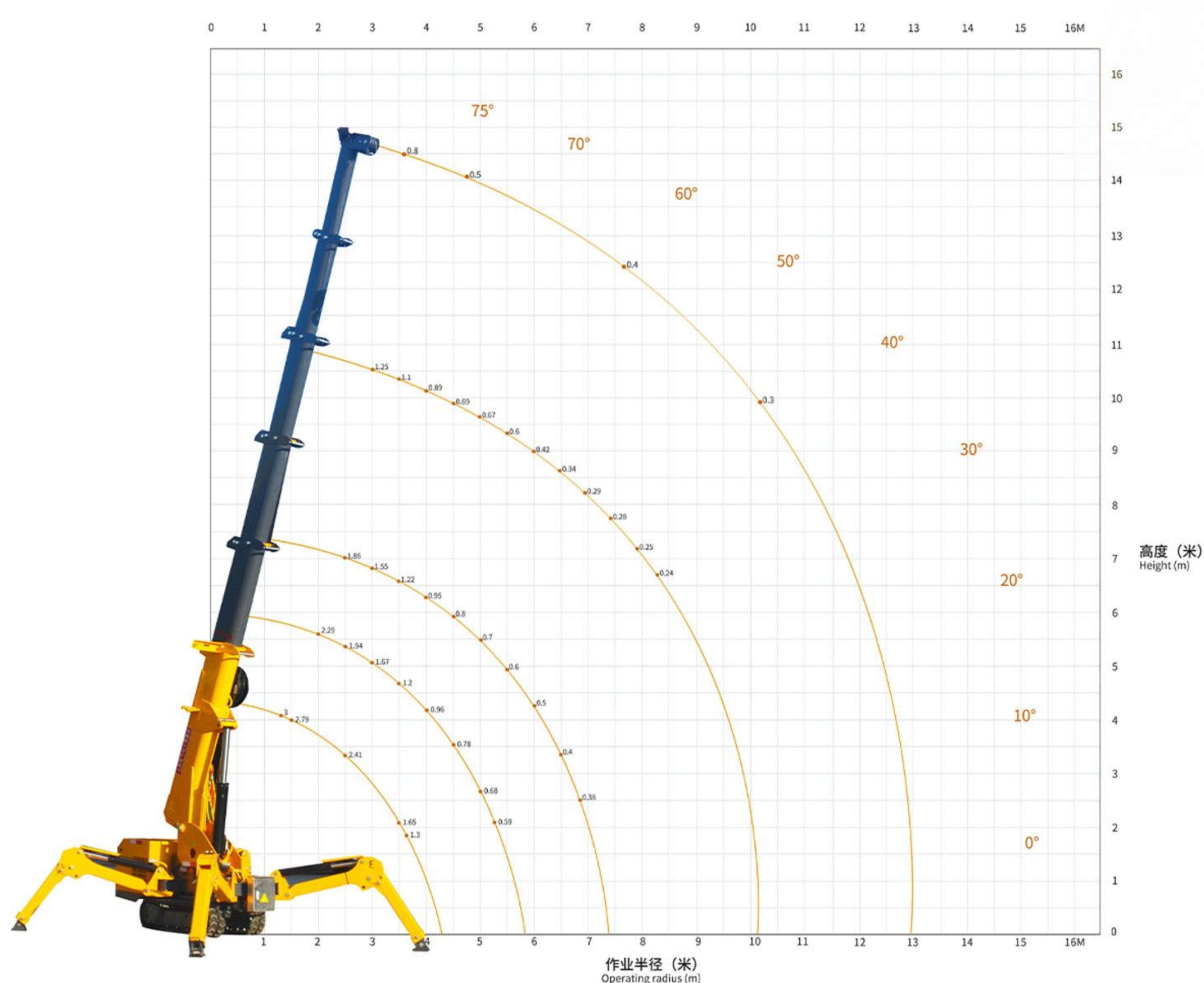
4吨蜘蛛吊重表 4 ton spider crane lifting weight chart
