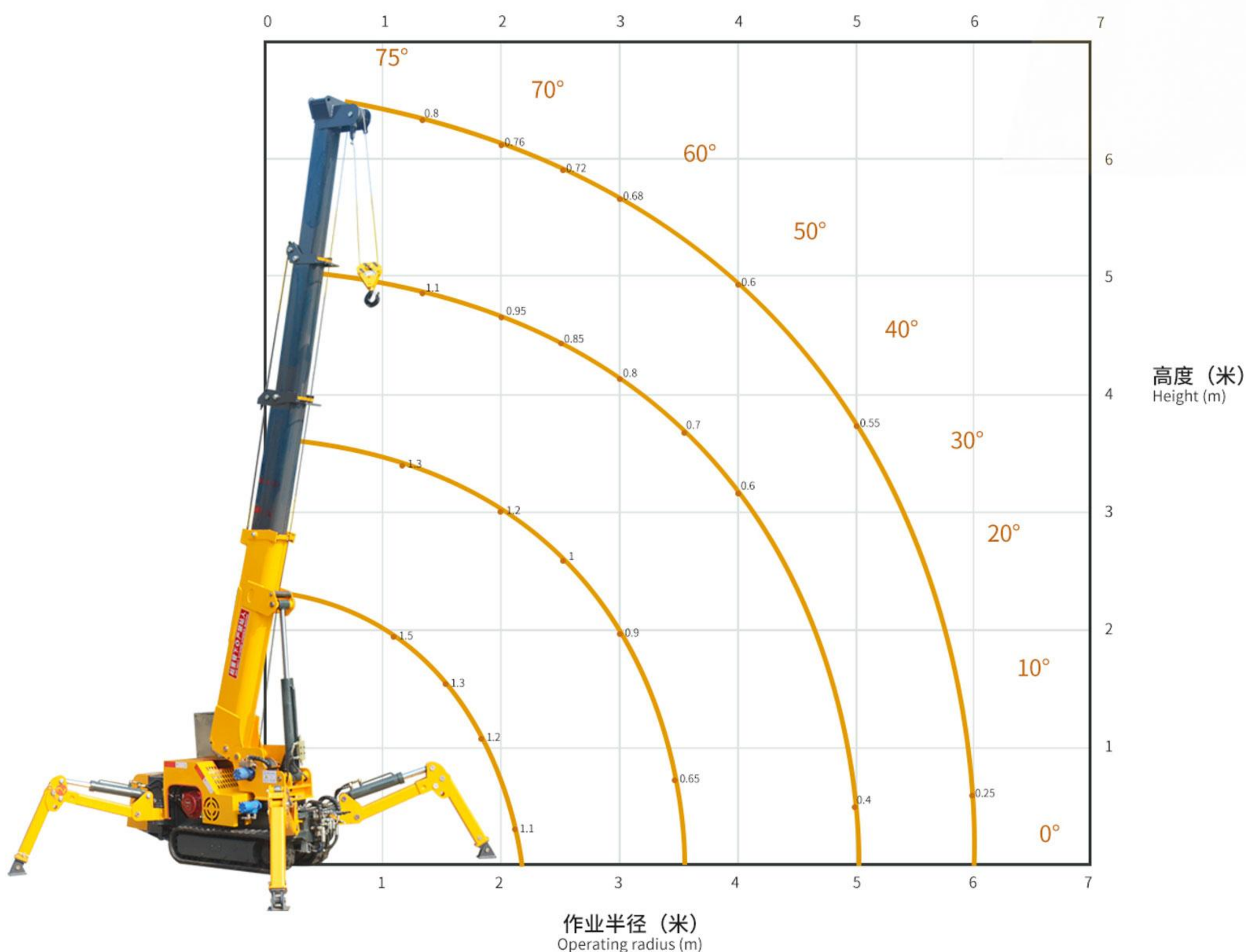
1.5吨蜘蛛吊吊重表 1.5 ton spider crane lifting weight chart
