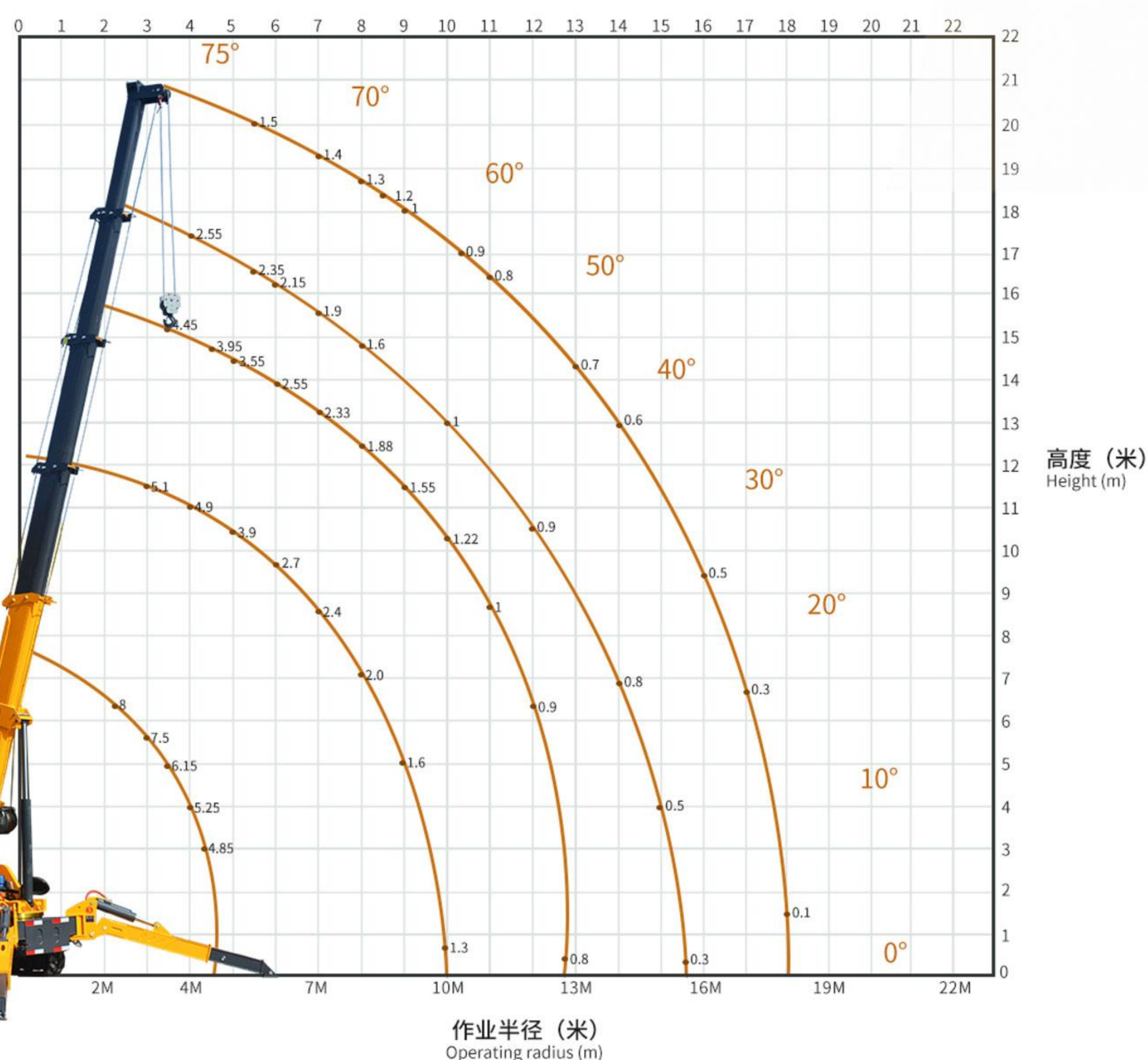
8吨蜘蛛吊机吊重表 8 ton spider crane lifting weight chart
